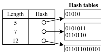
Fig. 2. Hash Tables for each possible prefix length
